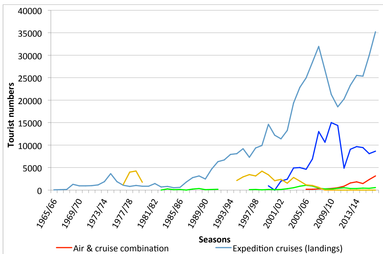
Figure 3.3. Antarctic tourism numbers (based on data obtained from IAATO, 2017)
